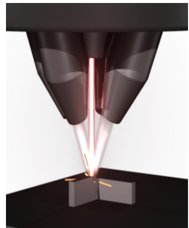
Figure 1: Artist's render of Directed Energy Deposition.
